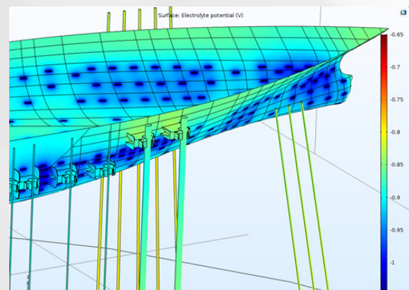
Ship hull protected by galvanic anodes
