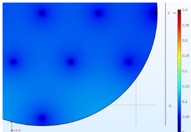
Tank bottom internal protected by galvanic anodes
