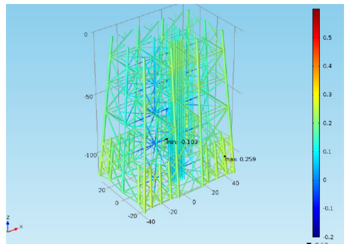
Platform jacket protected by impressed current system
