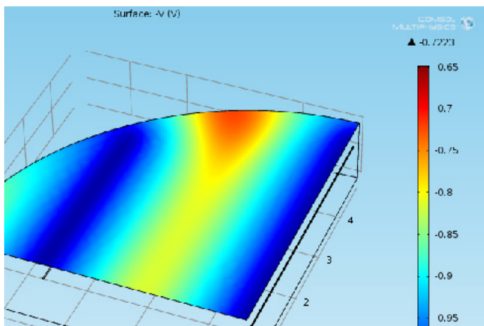
Tank bottom protected by 3 linear anodes
