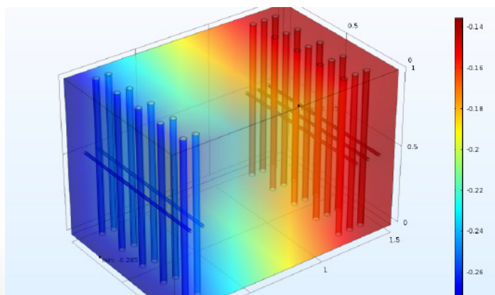
Potential distribution across reinforced concrete wall
