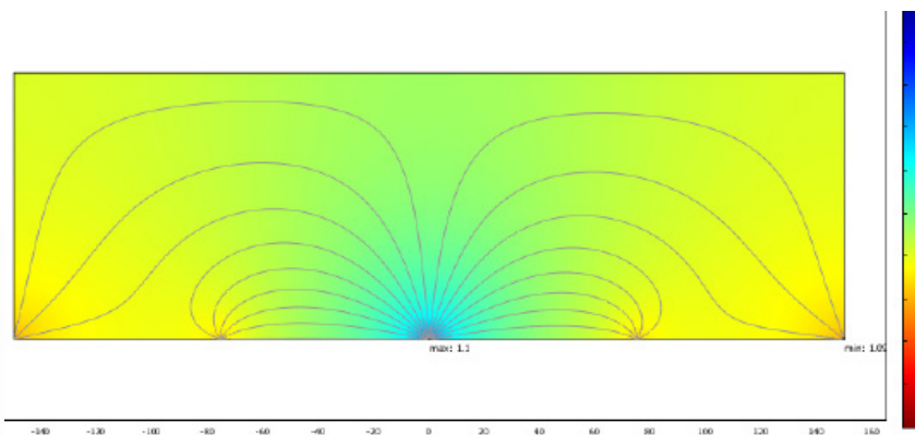
Simulation of 4 coating holidays on subsea pipeline
